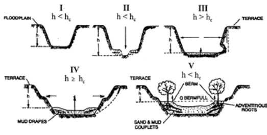
Figure 6 - Channel Changes Associated with Urbanization
