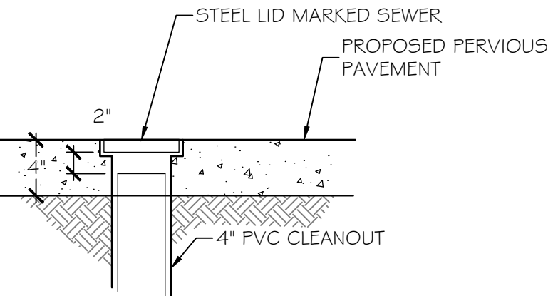
62 CLEANOUT DETAIL 'A' NTS
