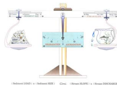
Figure 5 - Schematic of the Lane Relationship After Lane (1955) as cited in Rosgen (1996)
